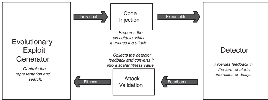
Fig. 1. EEG framework, which formulates the arms race.
